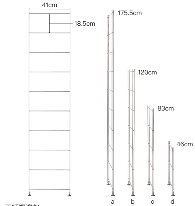
不銹鋼邊架 Stainless Steel Stand Panel
